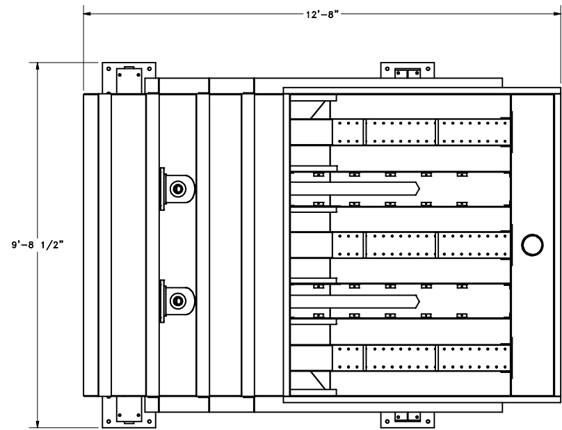
ASSEMBLY TOP VIEW SCALE 3/64
